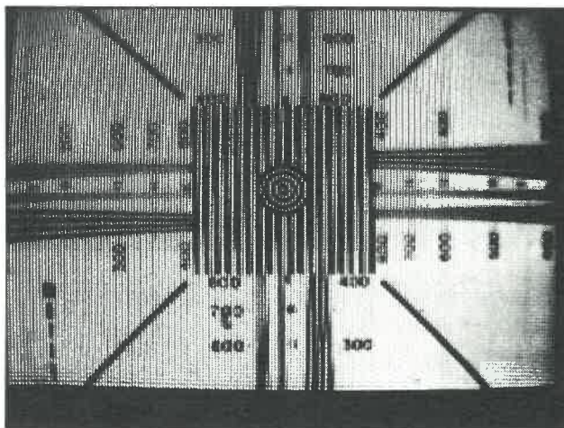
Figure 7. High light level images from (a) the DFGA and (b) FGA1 (To read the effective resolution, divide the test chart numbers by two.)
