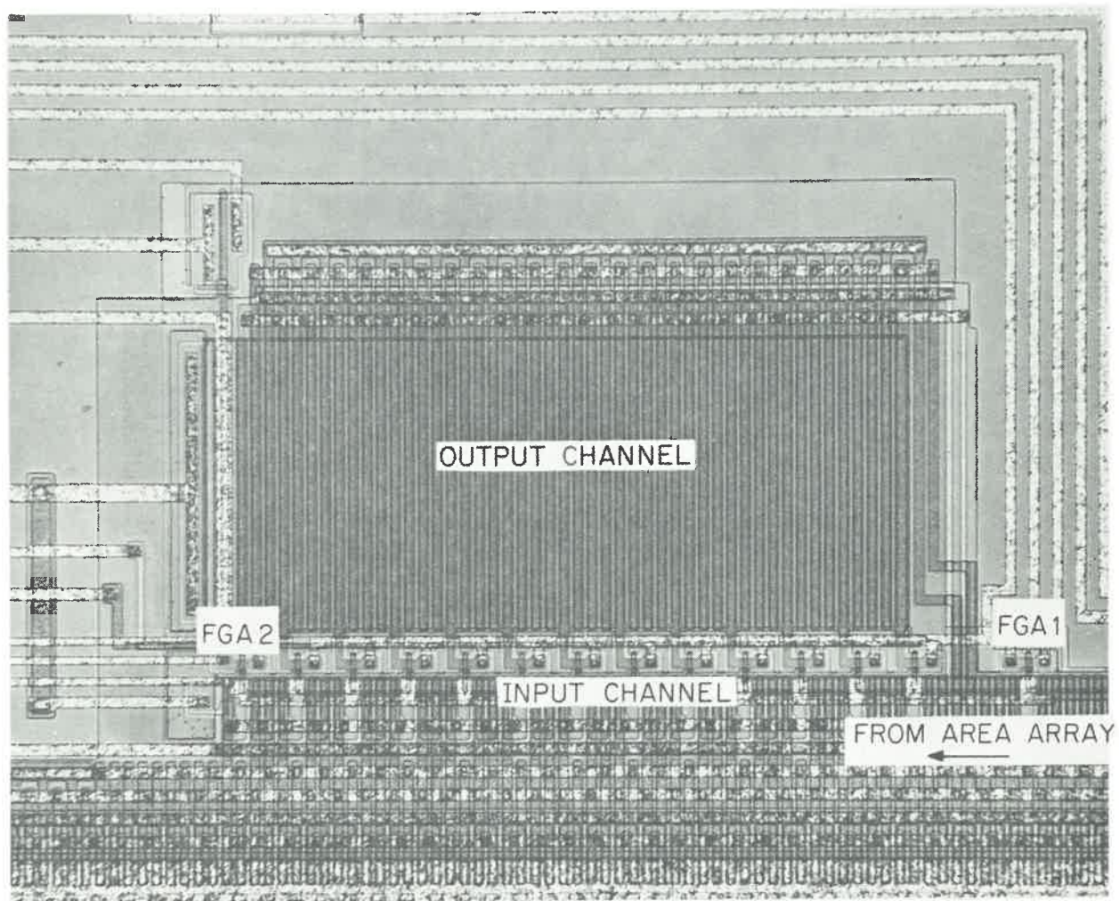
Figure 4. Floating-gate amplifier system
