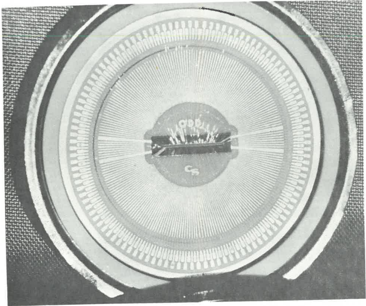
Figure 2. Multilayer ceramic header for a 212-channel Digicon
