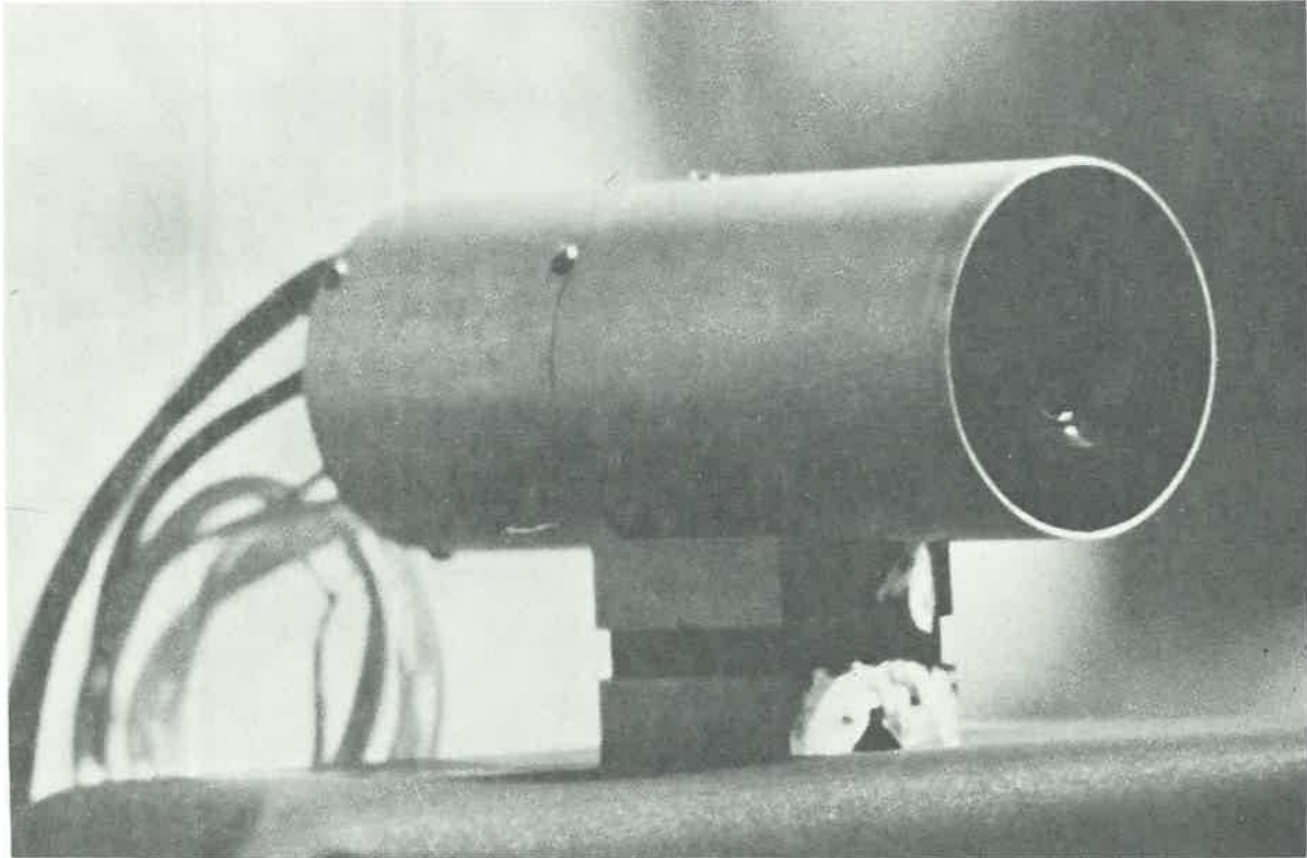
Figure 5. Quadrant Photosil for autoguiding on faint images
