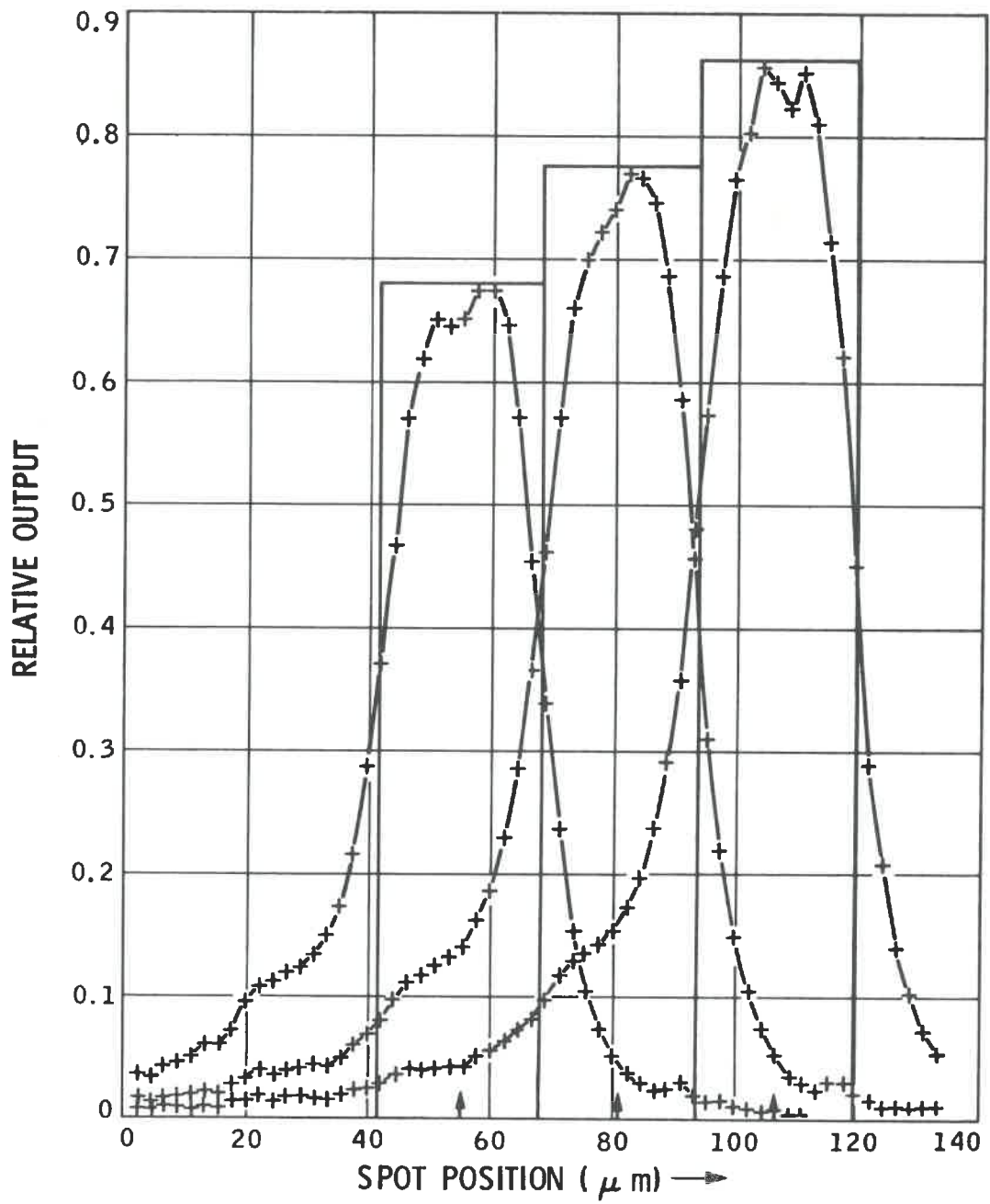
Figure 11. Sensitivity profile for three adjacent pixels (blue filter) (scan \perp to vertical channel)
