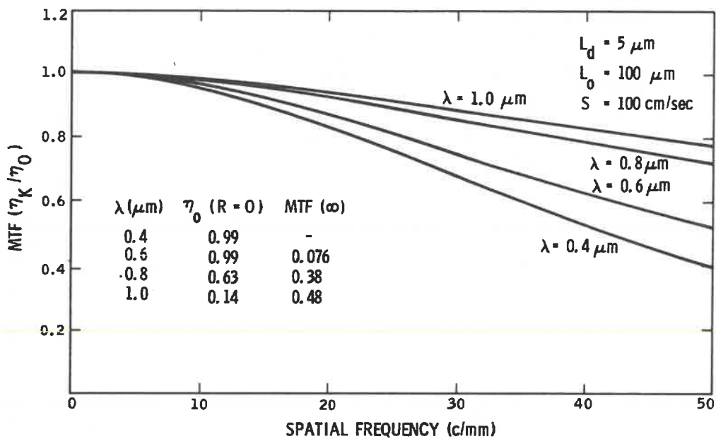
Figure 3. MTF for lateral diffusion ( L_T = 10 \mu\text{m} )
