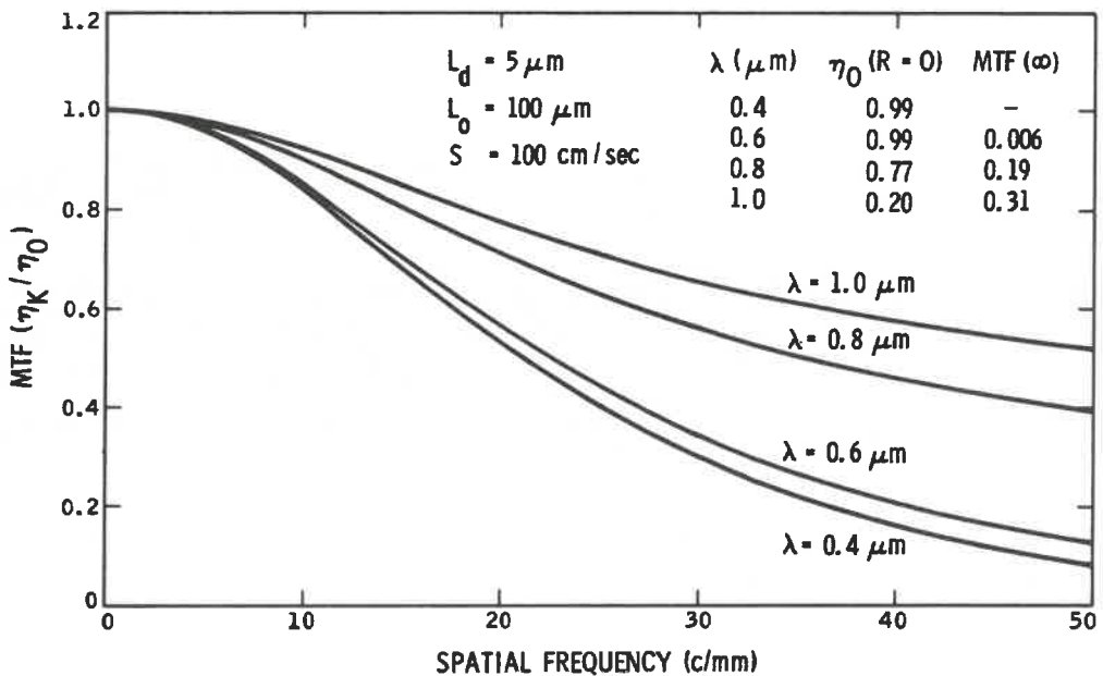
Figure 4. MTF for lateral diffusion ( L_T = 15 \mu\text{m} )
