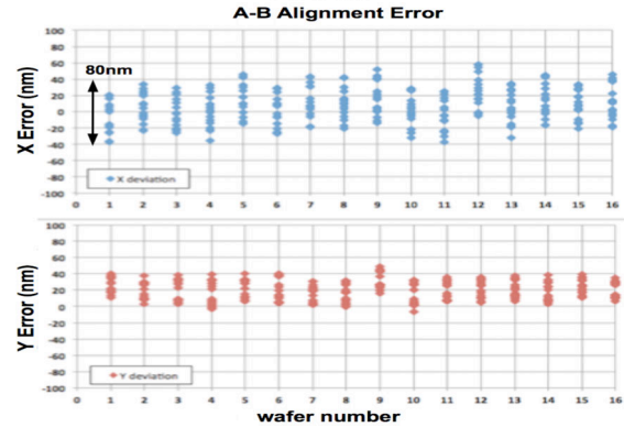
Fig. 4. Each CCD is stitched to connect the image array (A) and frame store (B), as shown on the above wafer image. The data shows X and Y alignment error between A-B fields. We achieve approximately 80-nm or better alignment error between fields in both directions across a sixteen wafer lot. This is well within the design requirements for a 15- \mu m pixel.
