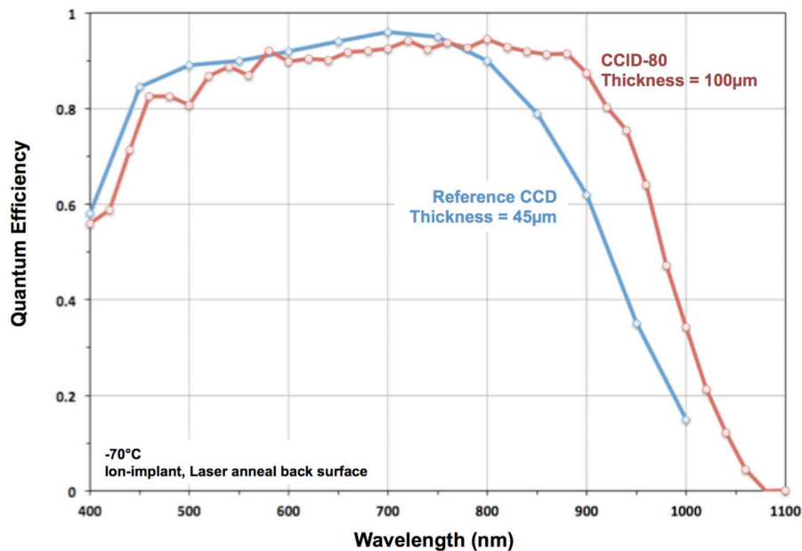
Fig. 8. Measured quantum efficiency for the 100-micron thick CCID-80 device compared to a 45-micron thick reference MIT LL CCD.
